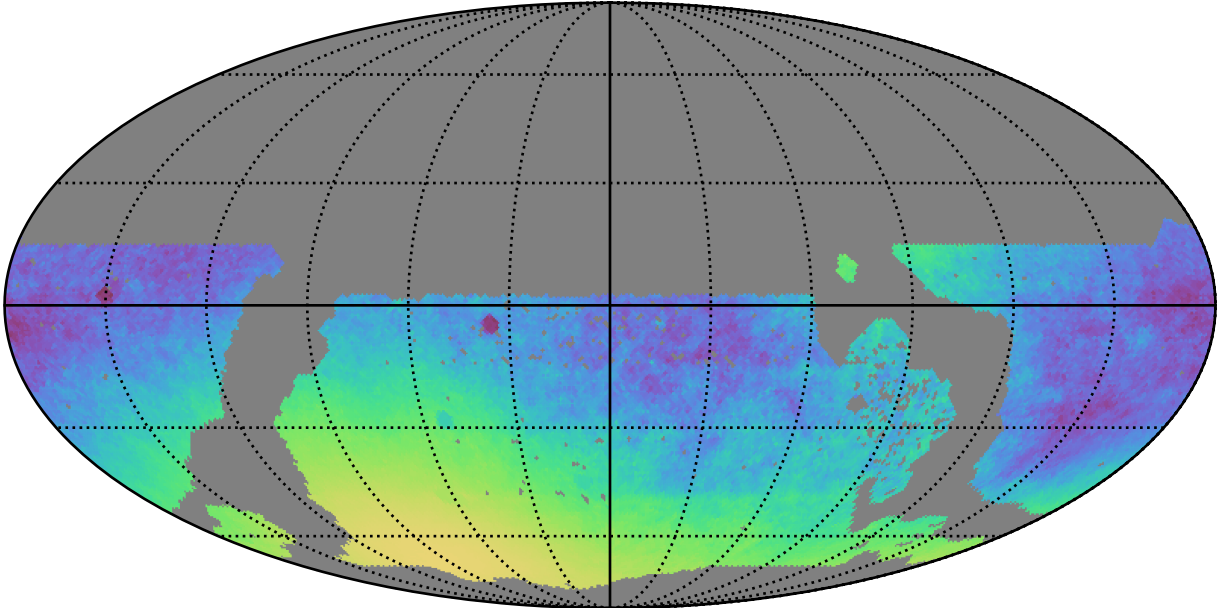
ddf_acor_sf20_lsf40_lsr10_v3.4_10yrs WFD y band only: Normalized Parallax Uncert @ 21.3
