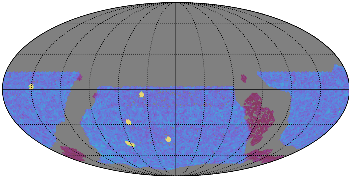
ddf_acor_sf20_lsf40_lsr10_v3.4_10yrs WFD y band: NVisits
