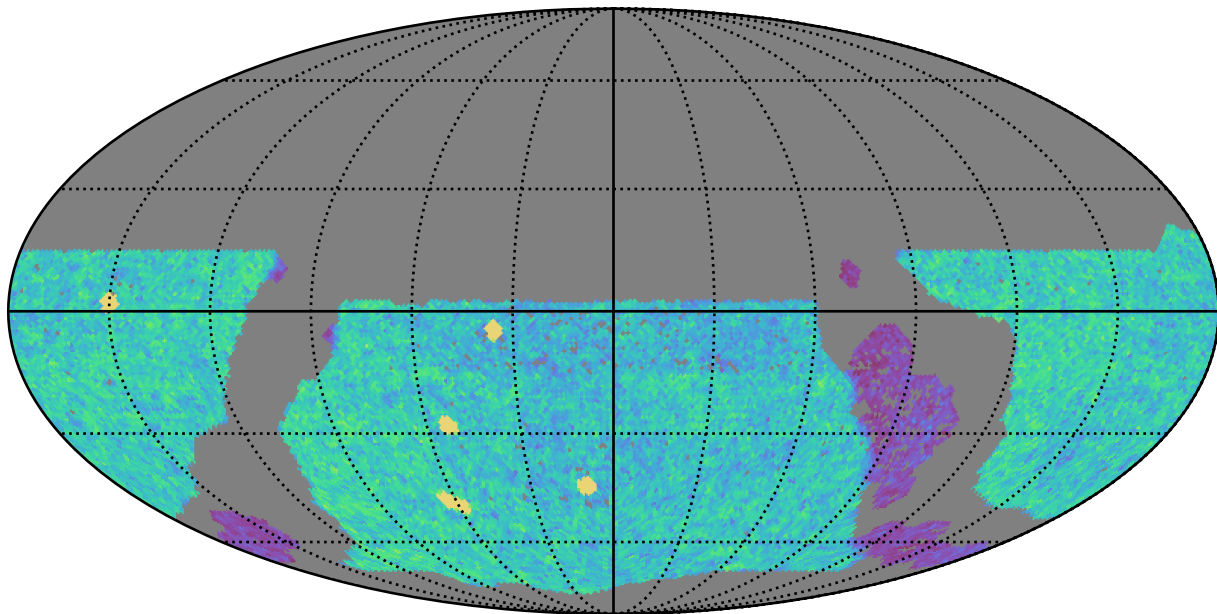
ddf_acor_sf20_lsf40_lsr10_v3.4_10yrs WFD u band: NVisits
