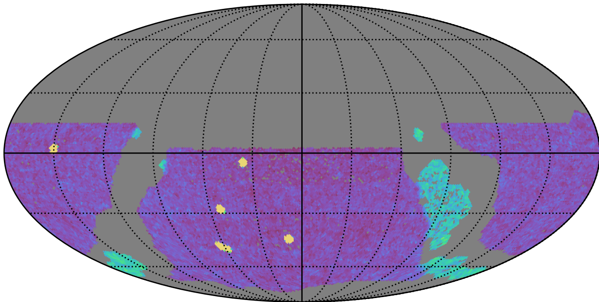
ddf_acor_sf20_lsf40_lsr10_v3.4_10yrs WFD g band: NVisits
