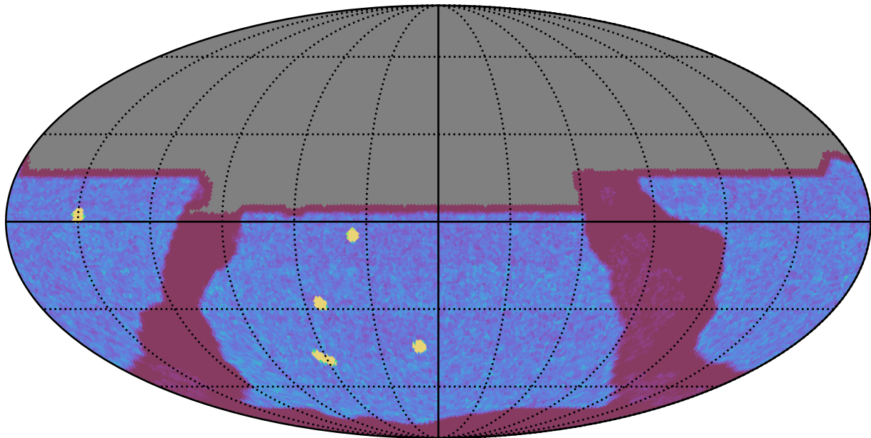
ddf_acor_sf20_lsf40_lsr10_v3.4_10yrs All sky y band: NVisits
