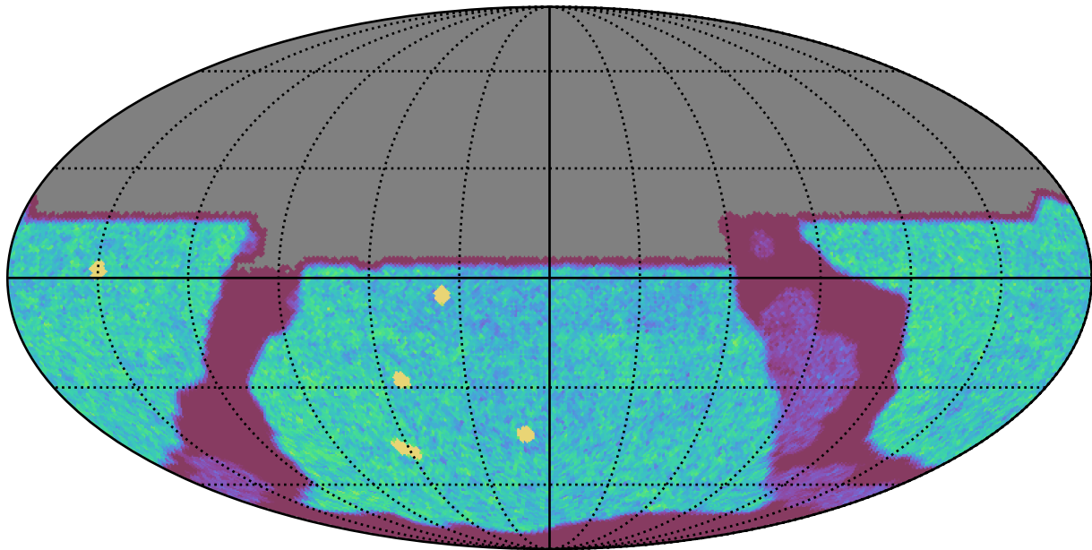
ddf_acor_sf20_lsf40_lsr10_v3.4_10yrs All sky u band: NVisits
