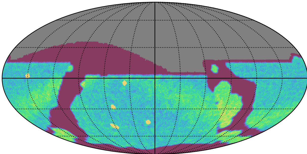
ddf_acor_sf20_lsf40_lsr10_v3.4_10yrs All sky r band: NVisits
