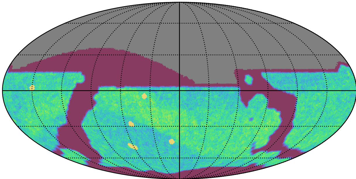
ddf_acor_sf20_lsf40_lsr10_v3.4_10yrs All sky i band: NVisits
