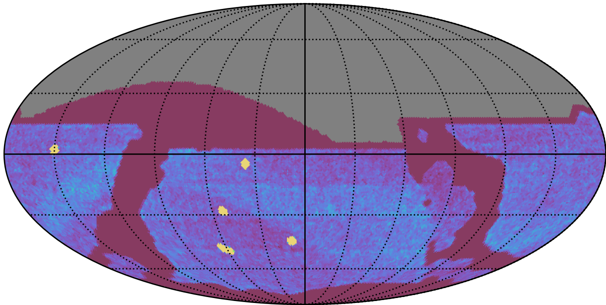
ddf_acor_sf20_lsf40_lsr10_v3.4_10yrs All sky all bands: NVisits
