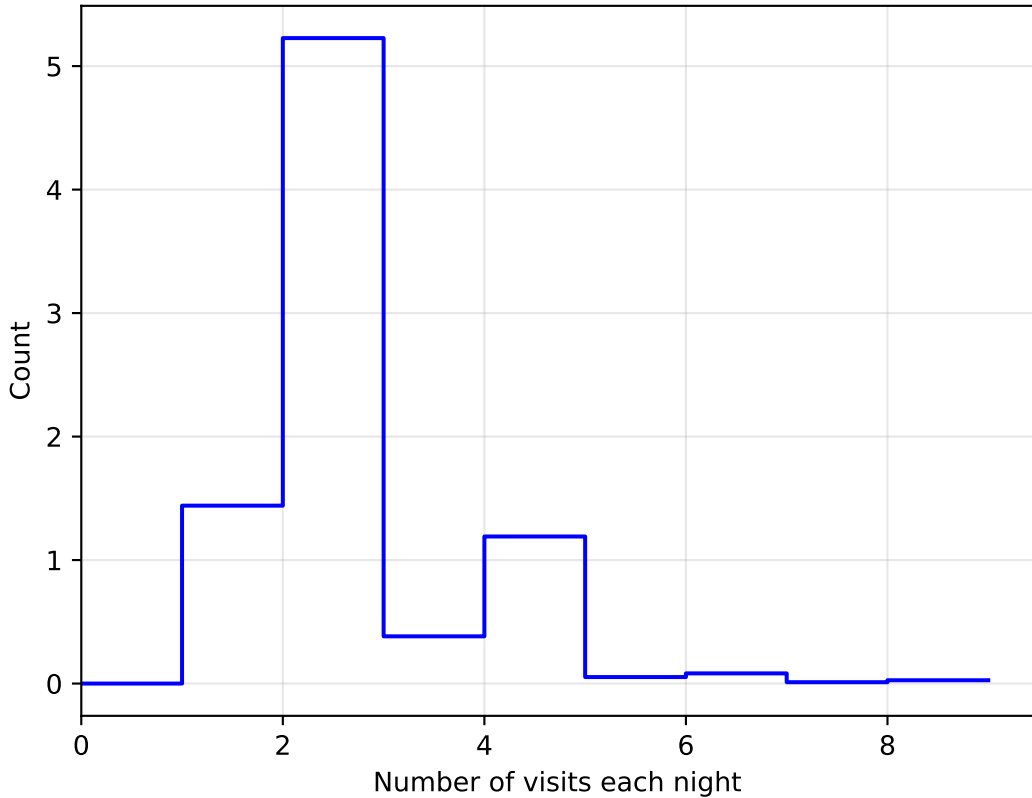
ddf_acor_sf20_lsf40_lsr10_v3.4_10yrs WFD: NVisitsPerNight 1e6
