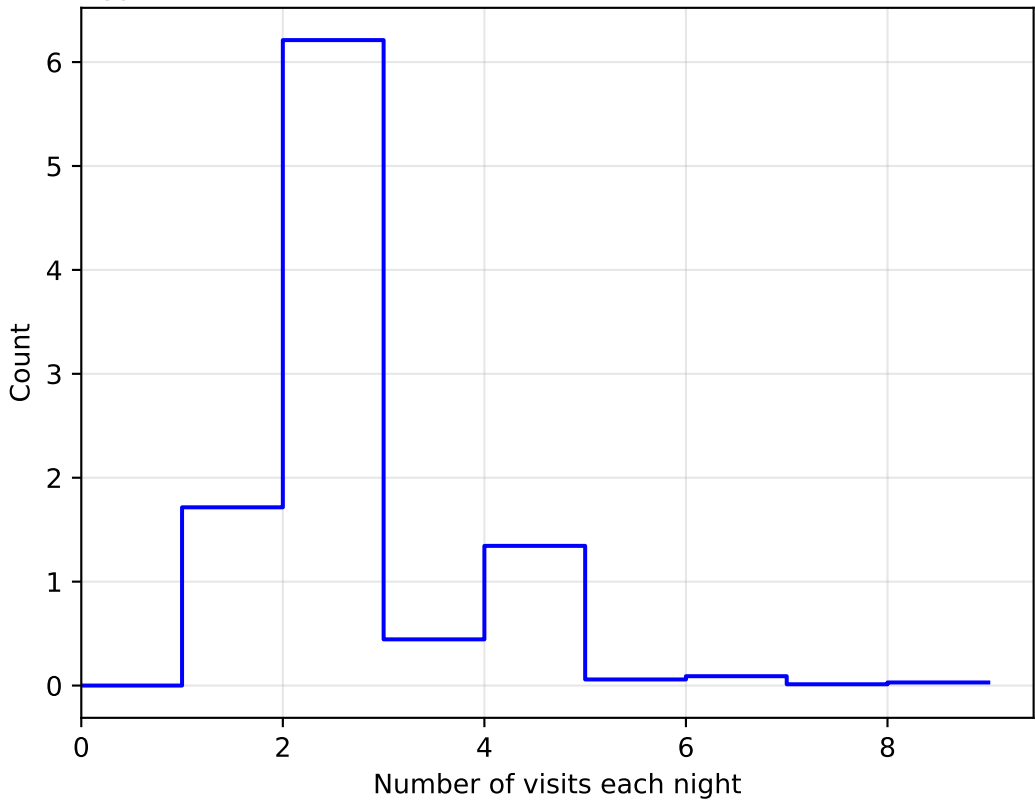
ddf_acor_sf20_lsf40_lsr10_v3.4_10yrs All sky: NVisitsPerNight 1e6
