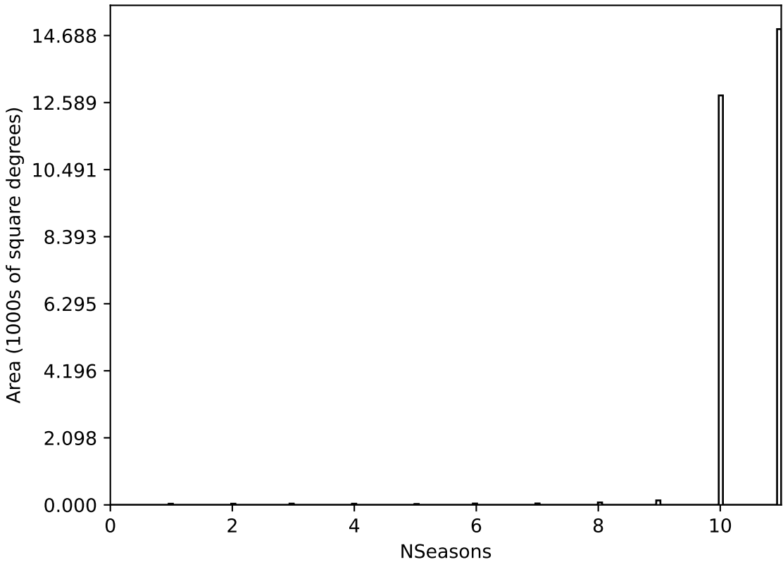
ddf_acor_sf20_lsf40_lsr10_v3.4_10yrs All sky all bands: NSeasons
