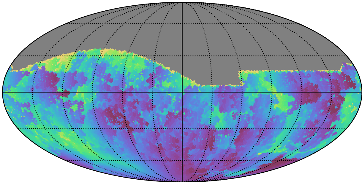
ddf_acor_sf20_lsf40_lsr10_v3.4_10yrs All sky g band: Min solarElong
