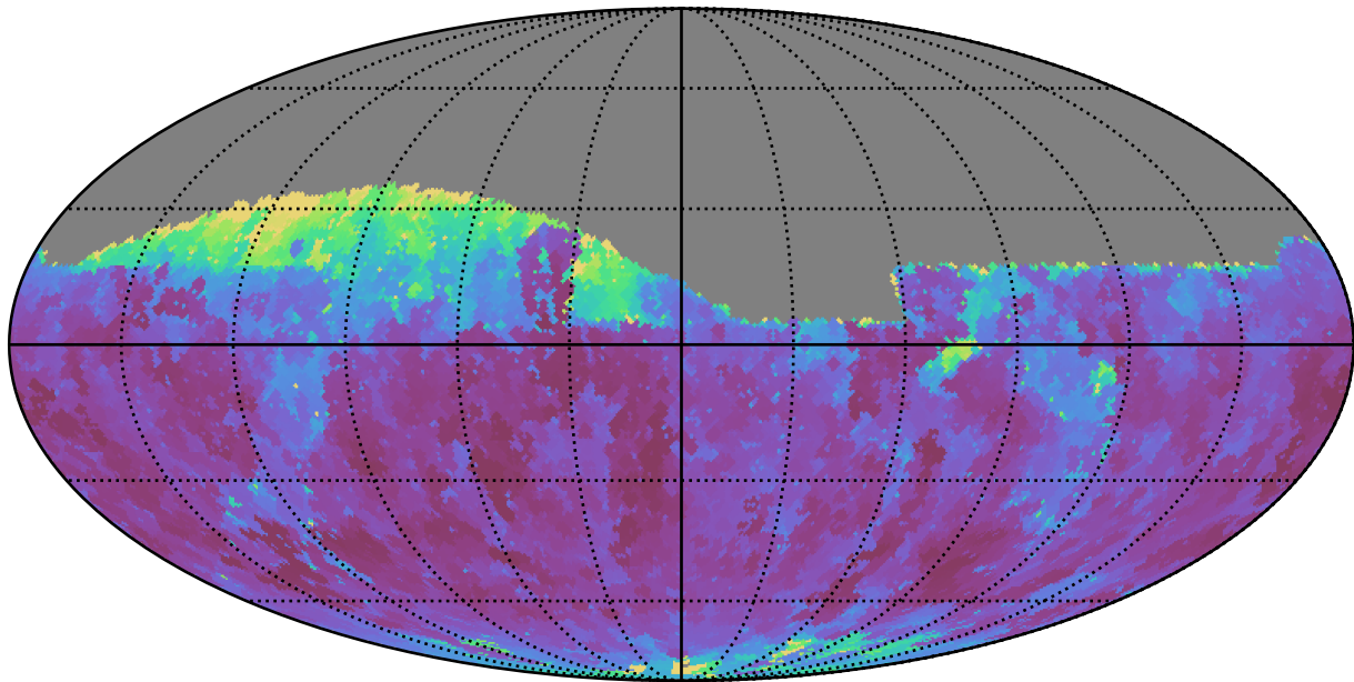
ddf_acor_sf20_lsf40_lsr10_v3.4_10yrs Yr 1 z band: Min seeingEff
