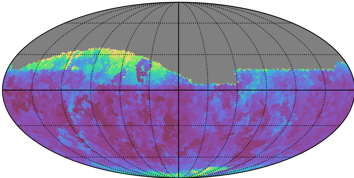
ddf_acor_sf20_lsf40_lsr10_v3.4_10yrs Yr 1 i band: Min seeingEff
