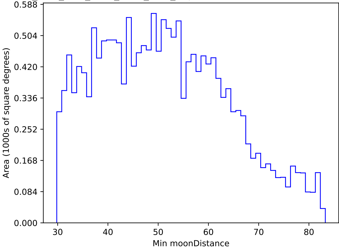
ddf_acor_sf20_lsf40_lsr10_v3.4_10yrs WFD u band: Min moonDistance
