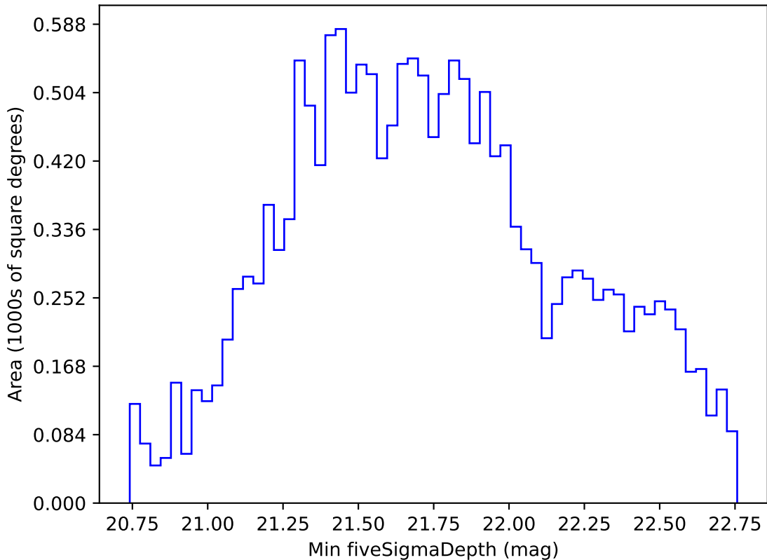
ddf_acor_sf20_lsf40_lsr10_v3.4_10yrs WFD i band: Min fiveSigmaDepth
