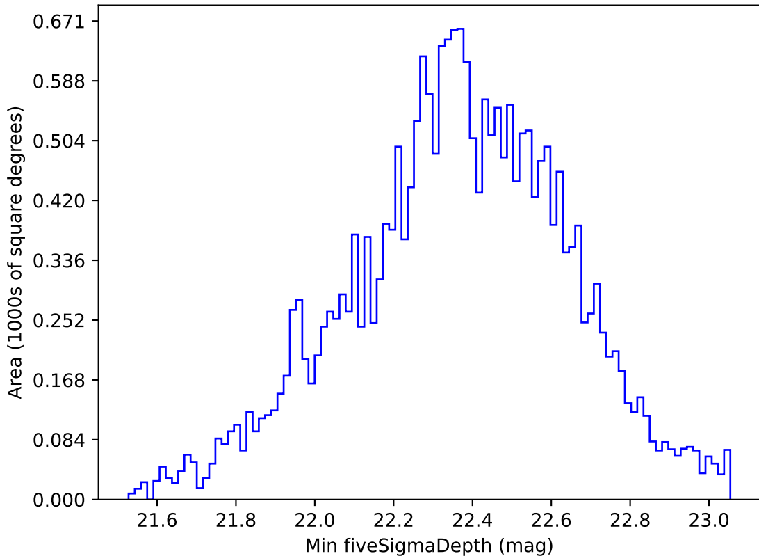
ddf_acor_sf20_lsf40_lsr10_v3.4_10yrs All sky u band: Min fiveSigmaDepth
