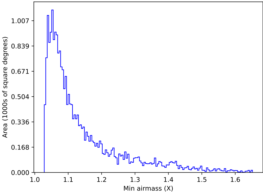
ddf_acor_sf20_lsf40_lsr10_v3.4_10yrs Yr 1 u band: Min airmass
