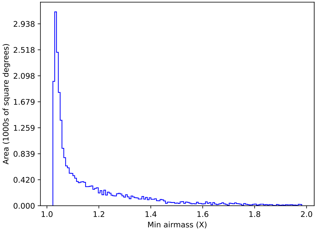
ddf_acor_sf20_lsf40_lsr10_v3.4_10yrs Yr 1 r band: Min airmass
