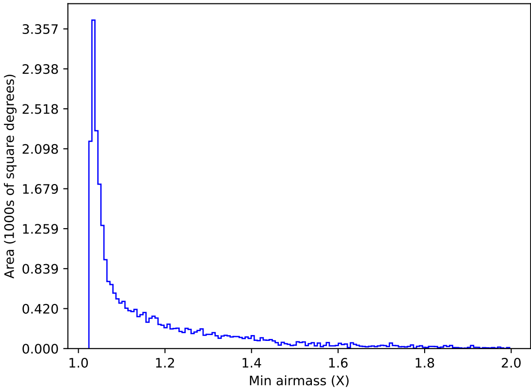
ddf_acor_sf20_lsf40_lsr10_v3.4_10yrs Yr 1 i band: Min airmass
