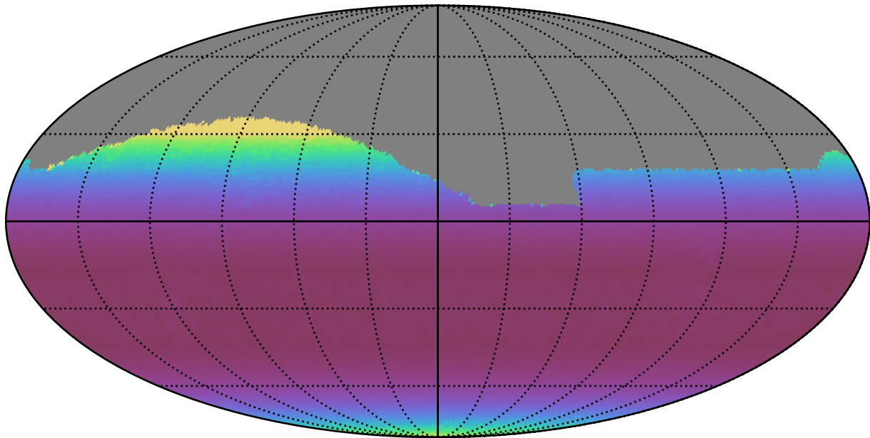
ddf_acor_sf20_lsf40_lsr10_v3.4_10yrs Yr 1 all bands: Min airmass
