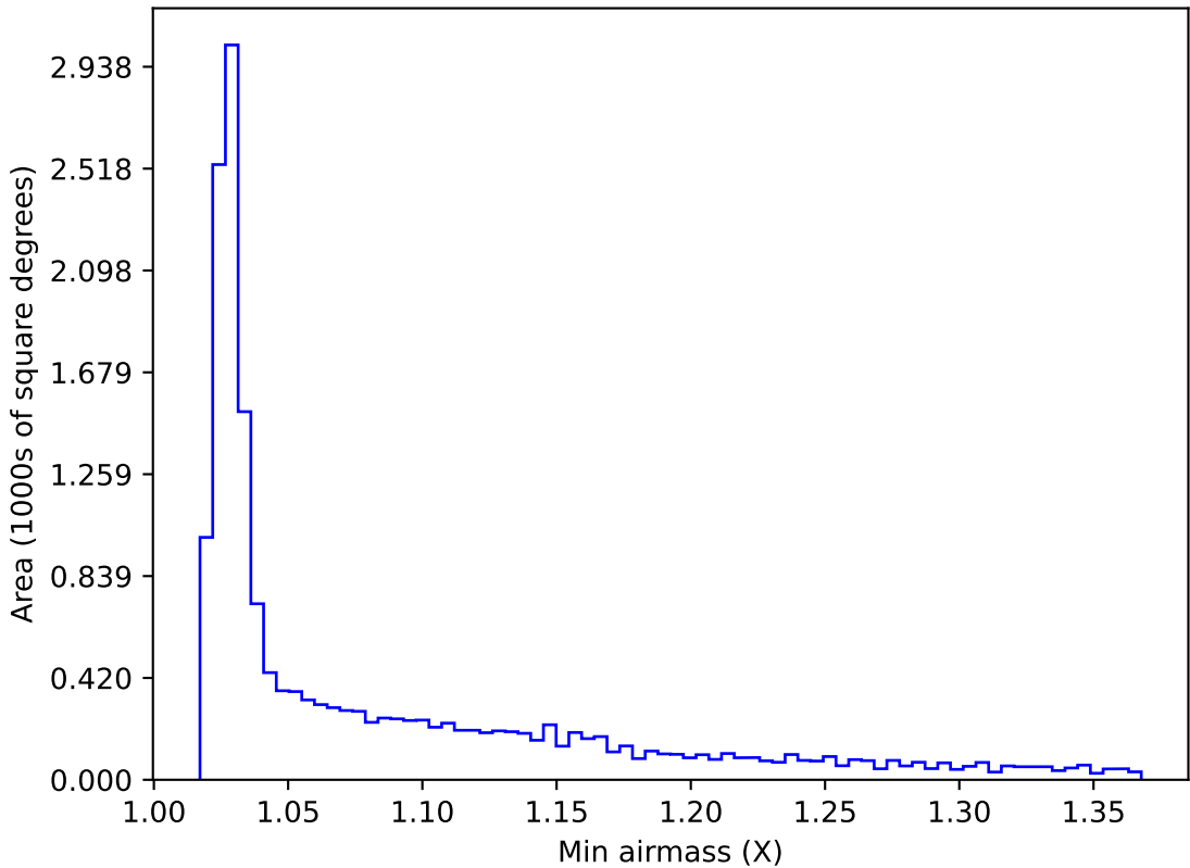
ddf_acor_sf20_lsf40_lsr10_v3.4_10yrs WFD r band: Min airmass
