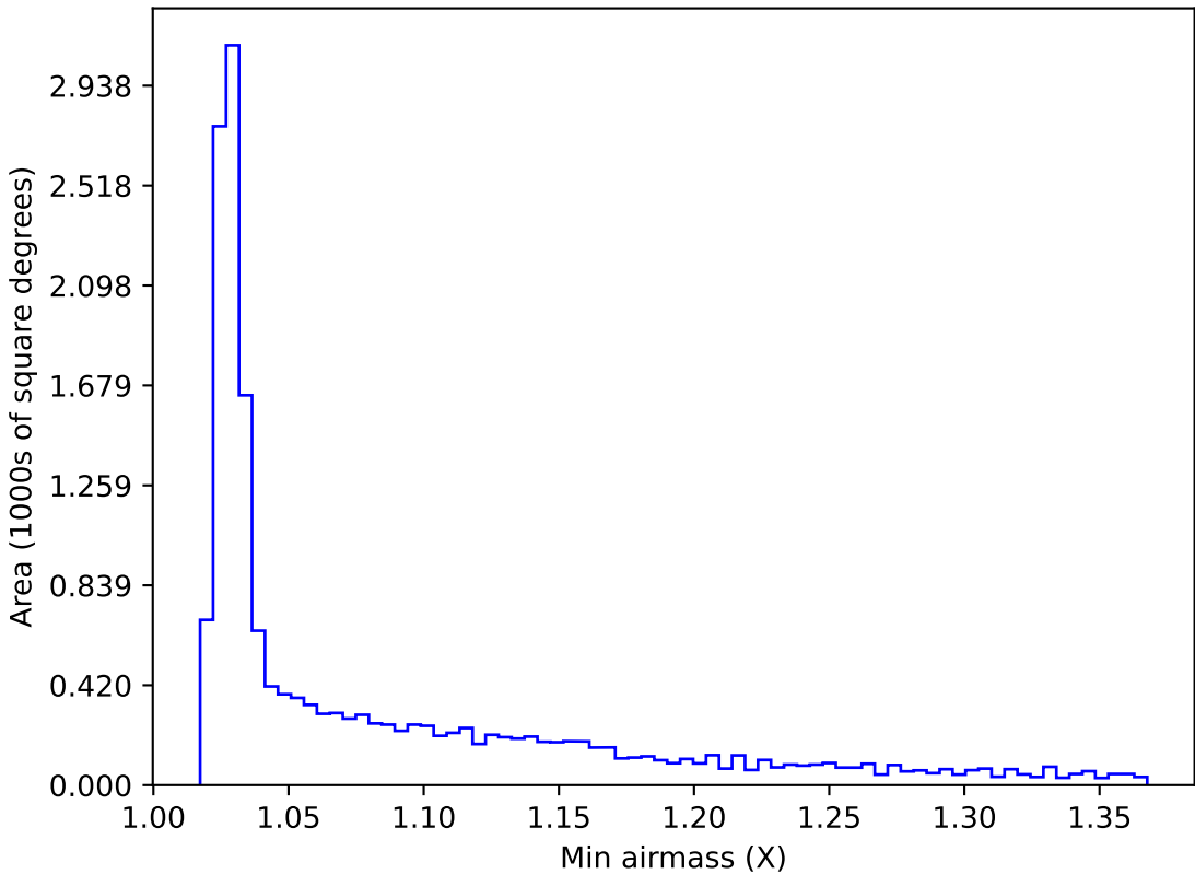
ddf_acor_sf20_lsf40_lsr10_v3.4_10yrs WFD i band: Min airmass
