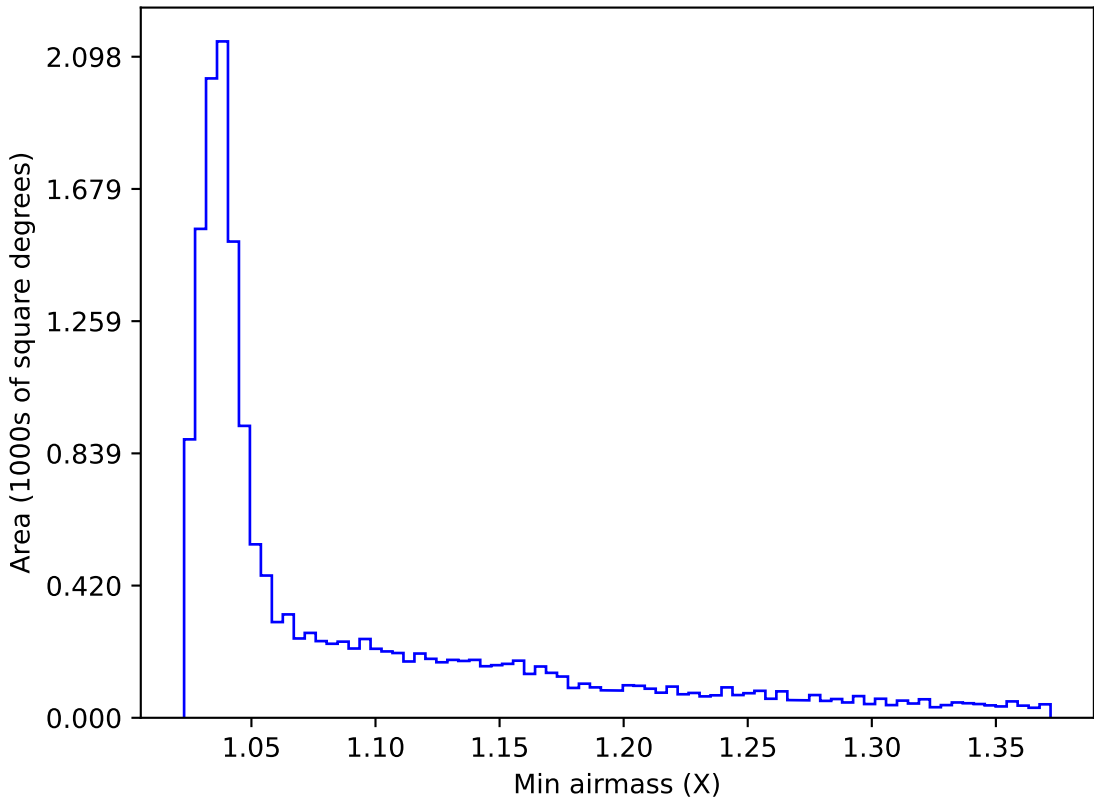
ddf_acor_sf20_lsf40_lsr10_v3.4_10yrs WFD g band: Min airmass
