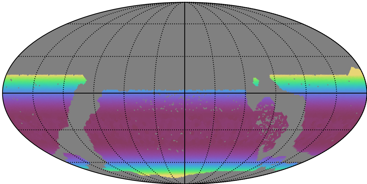
ddf_acor_sf20_lsf40_lsr10_v3.4_10yrs WFD all bands: Min airmass
