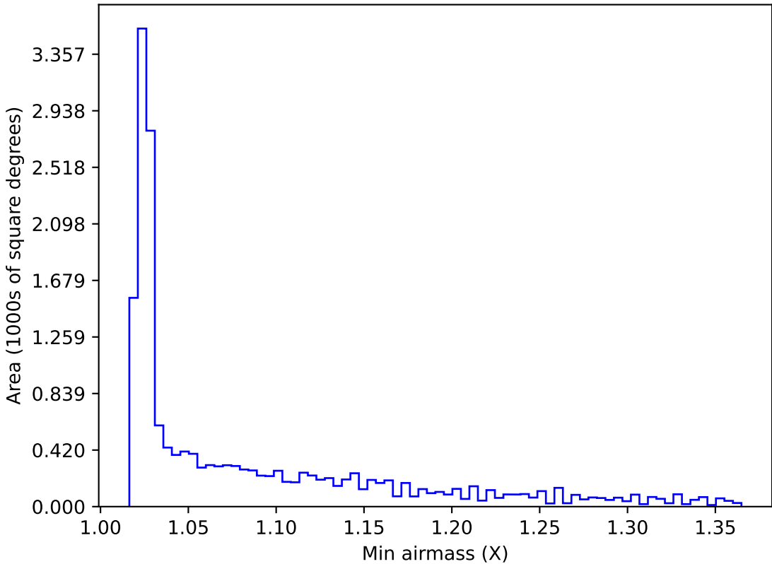
ddf_acor_sf20_lsf40_lsr10_v3.4_10yrs WFD all bands: Min airmass
