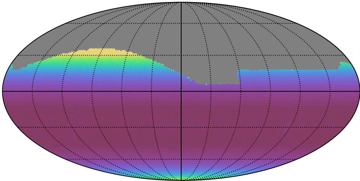
ddf_acor_sf20_lsf40_lsr10_v3.4_10yrs All sky r band: Min airmass
