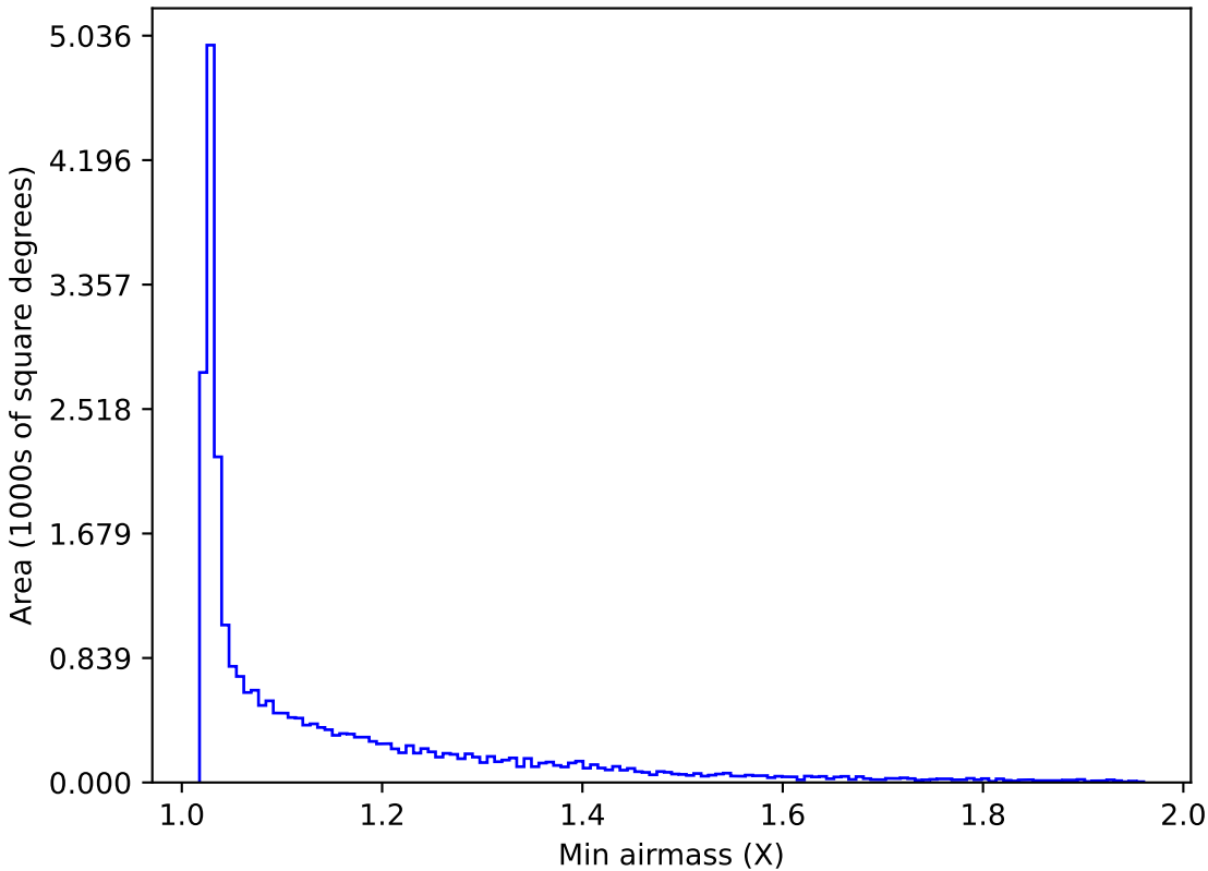
ddf_acor_sf20_lsf40_lsr10_v3.4_10yrs All sky r band: Min airmass
