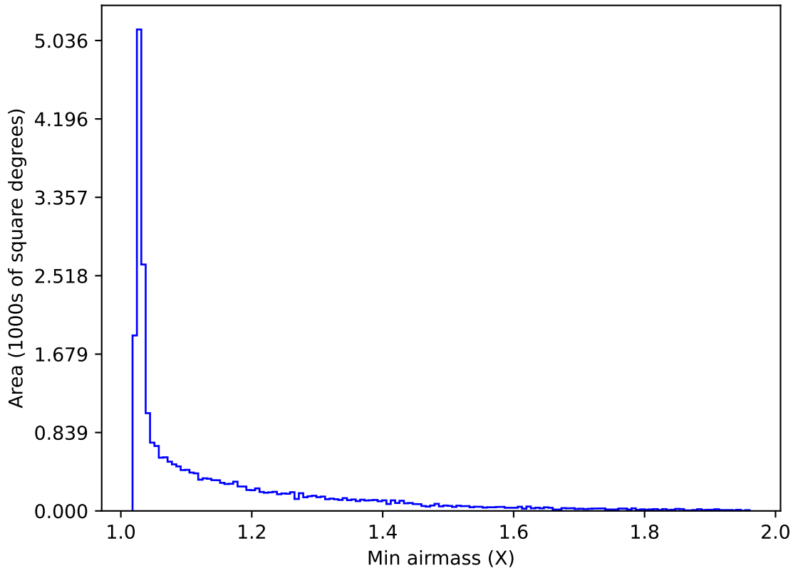
ddf_acor_sf20_lsf40_lsr10_v3.4_10yrs All sky i band: Min airmass
