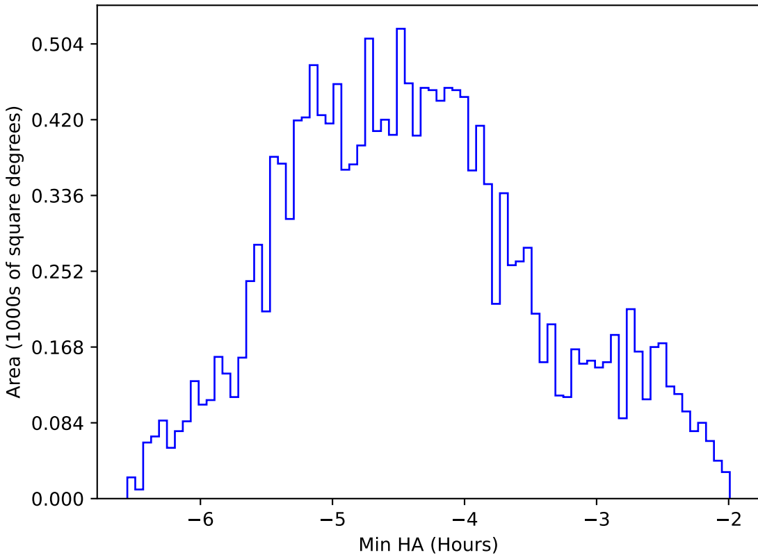
ddf_acor_sf20_lsf40_lsr10_v3.4_10yrs WFD z band: Min HA
