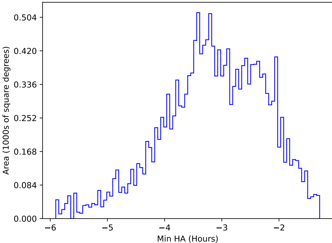
ddf_acor_sf20_lsf40_lsr10_v3.4_10yrs WFD u band: Min HA
