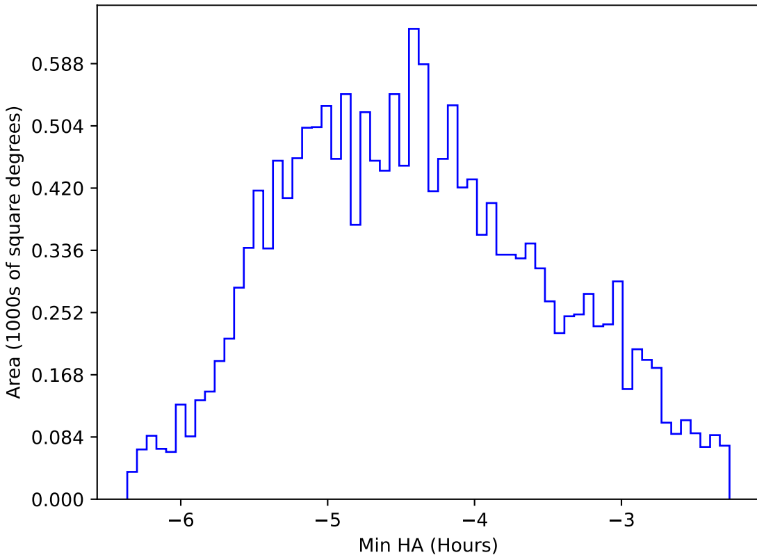
ddf_acor_sf20_lsf40_lsr10_v3.4_10yrs WFD r band: Min HA
