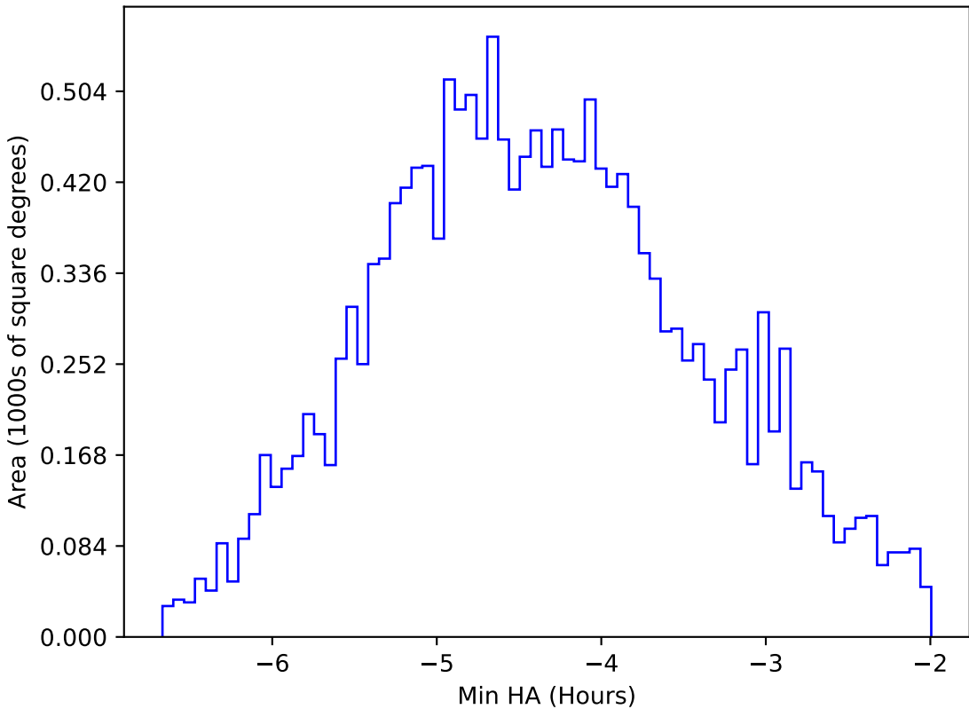
ddf_acor_sf20_lsf40_lsr10_v3.4_10yrs WFD i band: Min HA
