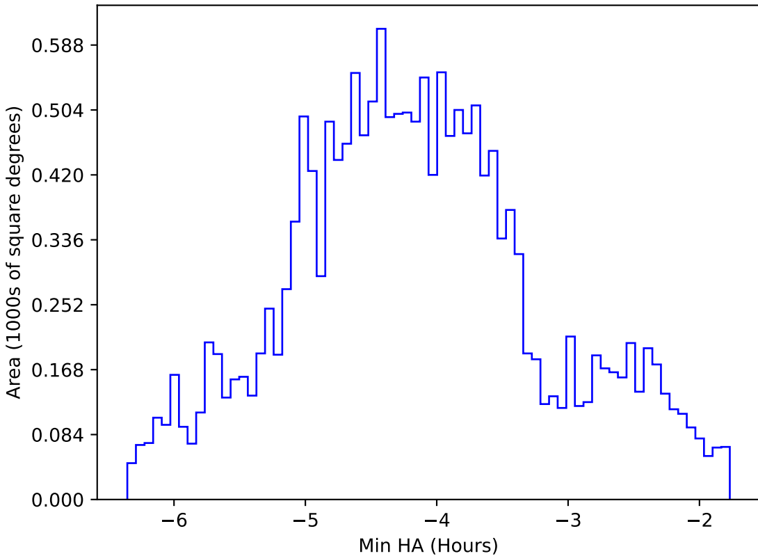
ddf_acor_sf20_lsf40_lsr10_v3.4_10yrs WFD g band: Min HA
