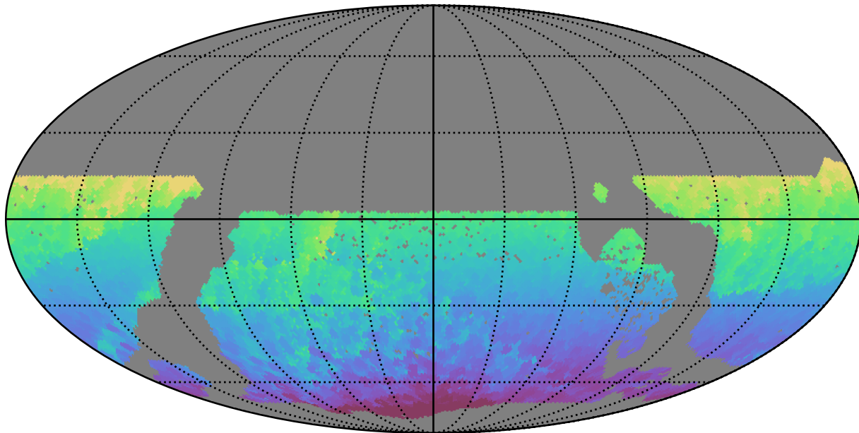
ddf_acor_sf20_lsf40_lsr10_v3.4_10yrs WFD all bands: Min HA
