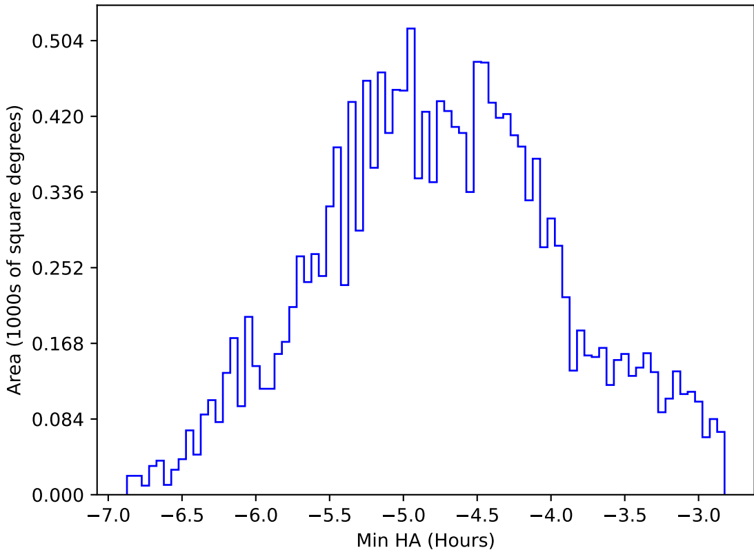
ddf_acor_sf20_ls40_lsr10_v3.4_10yrs WFD all bands: Min HA
