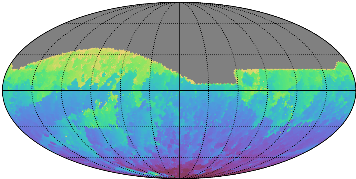
ddf_acor_sf20_lsf40_lsr10_v3.4_10yrs All sky z band: Min HA
