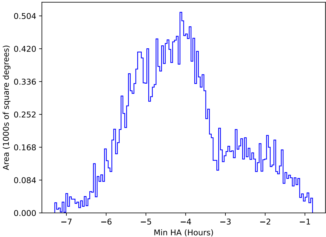
ddf_acor_sf20_lsf40_lsr10_v3.4_10yrs All sky z band: Min HA
