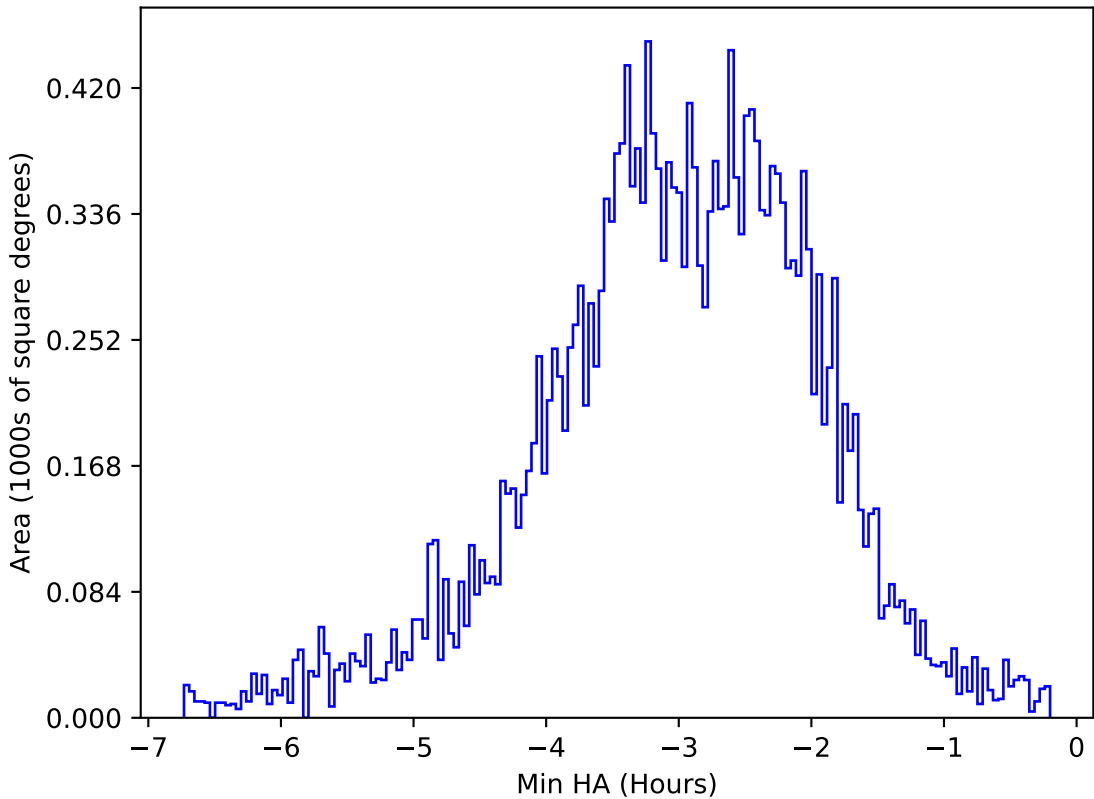
ddf_acor_sf20_lsf40_lsr10_v3.4_10yrs All sky u band: Min HA
