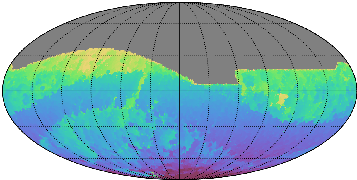
ddf_acor_sf20_lsf40_lsr10_v3.4_10yrs All sky r band: Min HA
