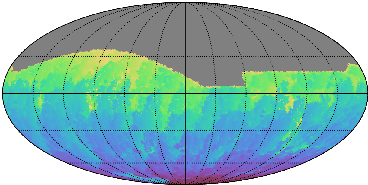
ddf_acor_sf20_lsf40_lsr10_v3.4_10yrs All sky g band: Min HA
