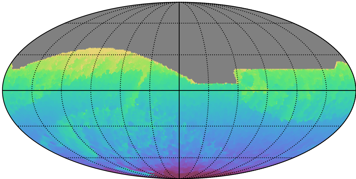
ddf_acor_sf20_lsf40_lsr10_v3.4_10yrs All sky all bands: Min HA
