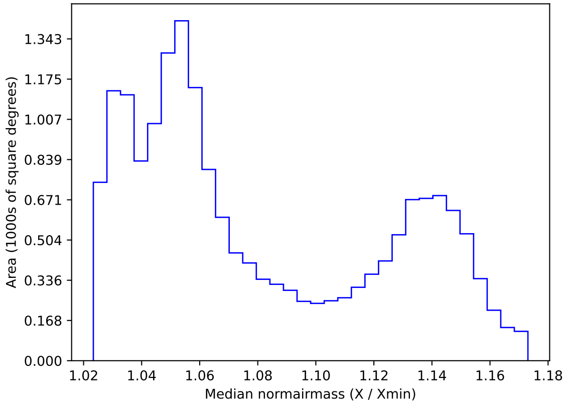
ddf_acor_sf20_lsf40_lsr10_v3.4_10yrs WFD all bands: Median normairmass
