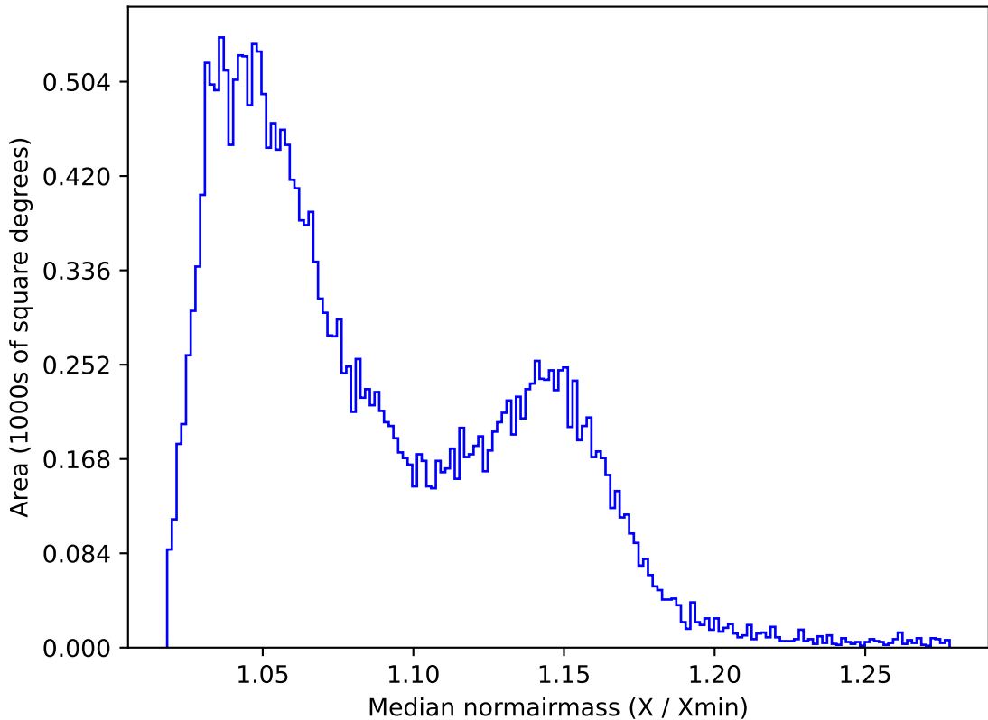
ddf_acor_sf20_ls40_lsr10_v3.4_10yrs All sky z band: Median normairmass
