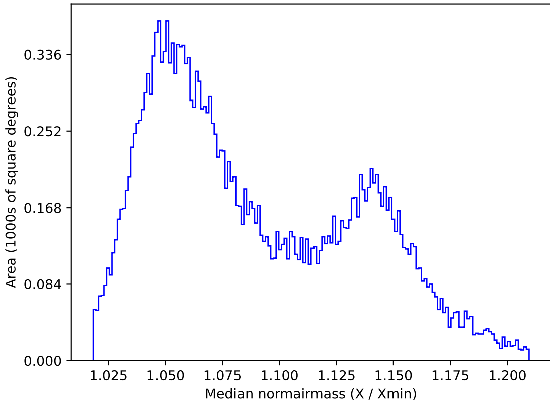
ddf_acor_sf20_ls40_lsr10_v3.4_10yrs All sky y band: Median normairmass
