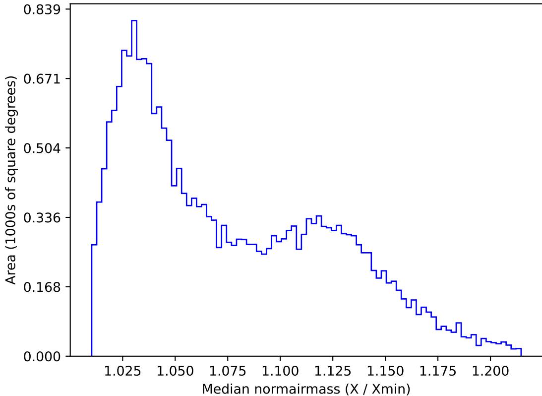
ddf_acor_sf20_lsf40_lsr10_v3.4_10yrs All sky u band: Median normairmass
