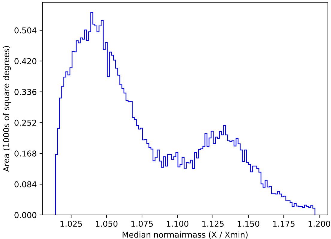
ddf_acor_sf20_lsf40_lsr10_v3.4_10yrs All sky r band: Median normairmass
