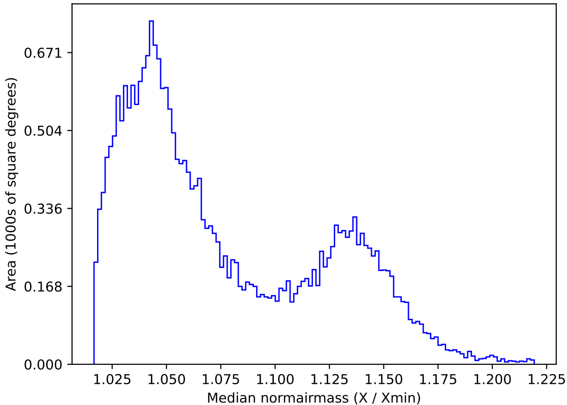
ddf_acor_sf20_lsf40_lsr10_v3.4_10yrs All sky i band: Median normairmass
