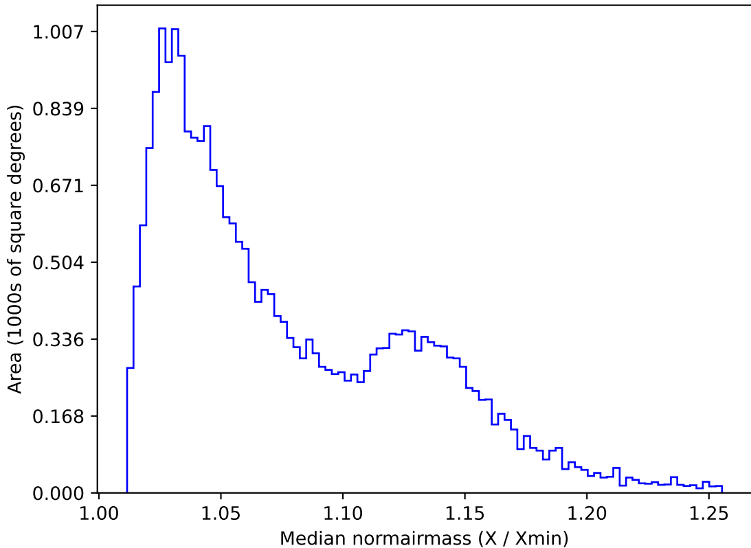
ddf_acor_sf20_lsf40_lsr10_v3.4_10yrs All sky g band: Median normairmass
